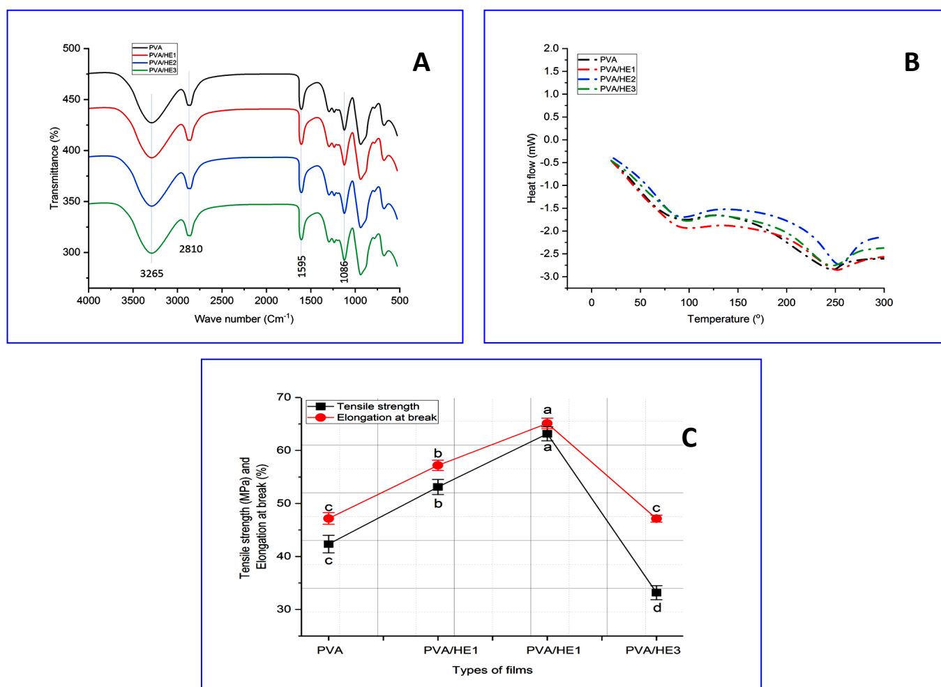
Figure 2. FT-IR spectra (A), DSC curves (B) and mechanical properties (C) of PVA/HE films
